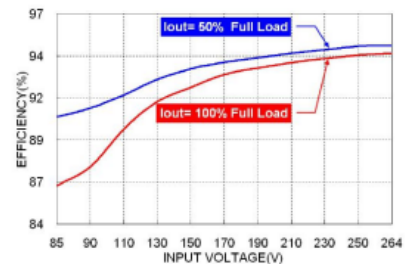
Efficiency vs. Input Voltage 43T□H450US24 with Forced air cooling
